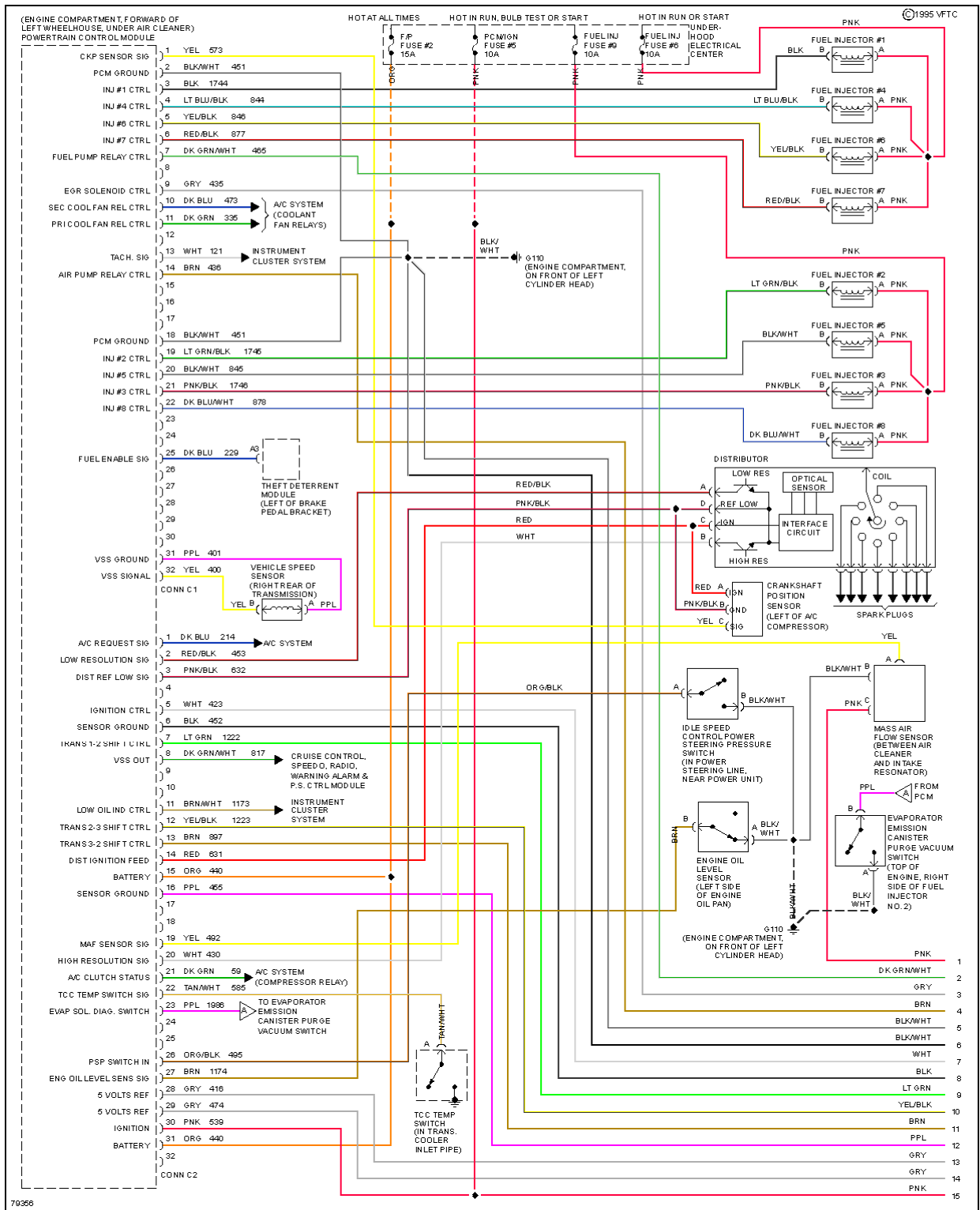
Fig. 9: 5.7L (VIN P), Engine Performance Circuits (1 of 3)
