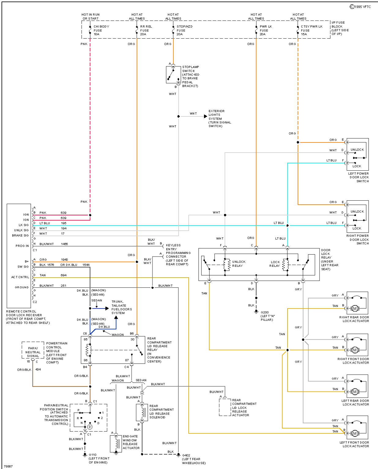
Fig. 32: Keyless Entry Circuit
