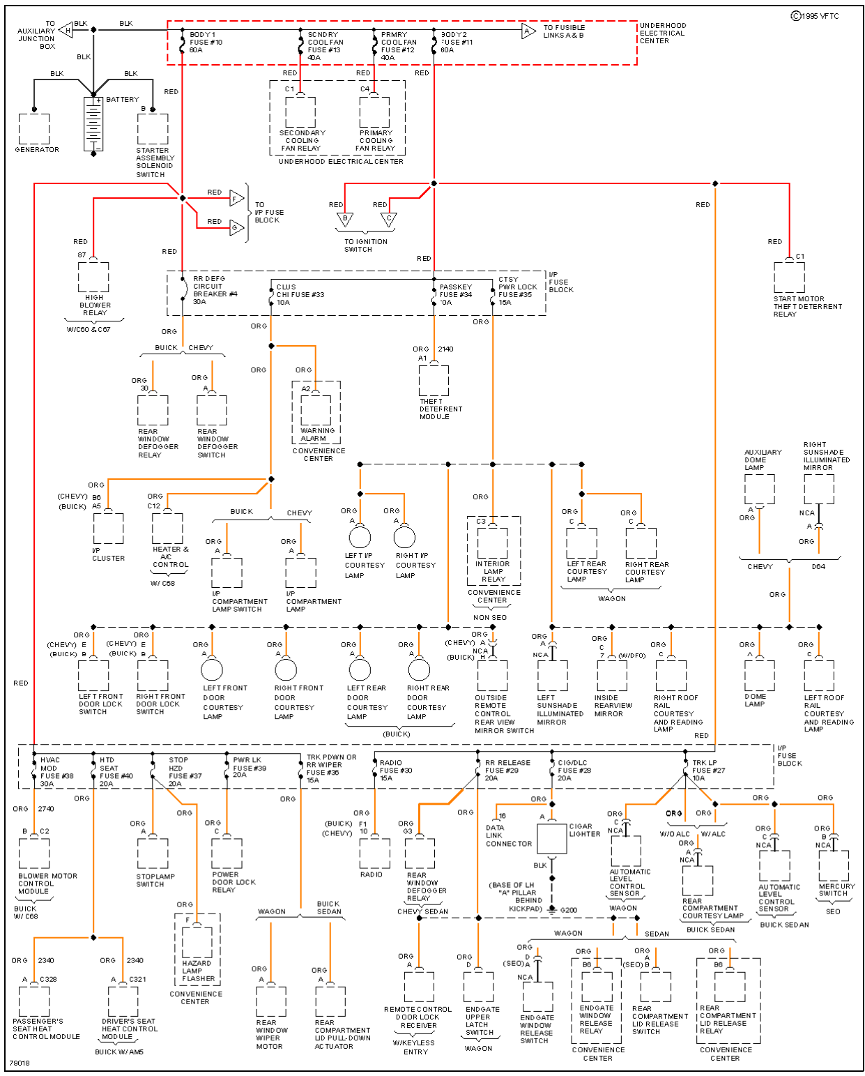
Fig. 27: Power Distribution Circuit (1 of 4)
