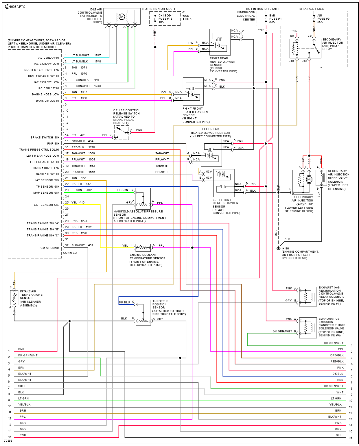
Fig. 10: 5.7L (VIN P), Engine Performance Circuits (2 of 3)
