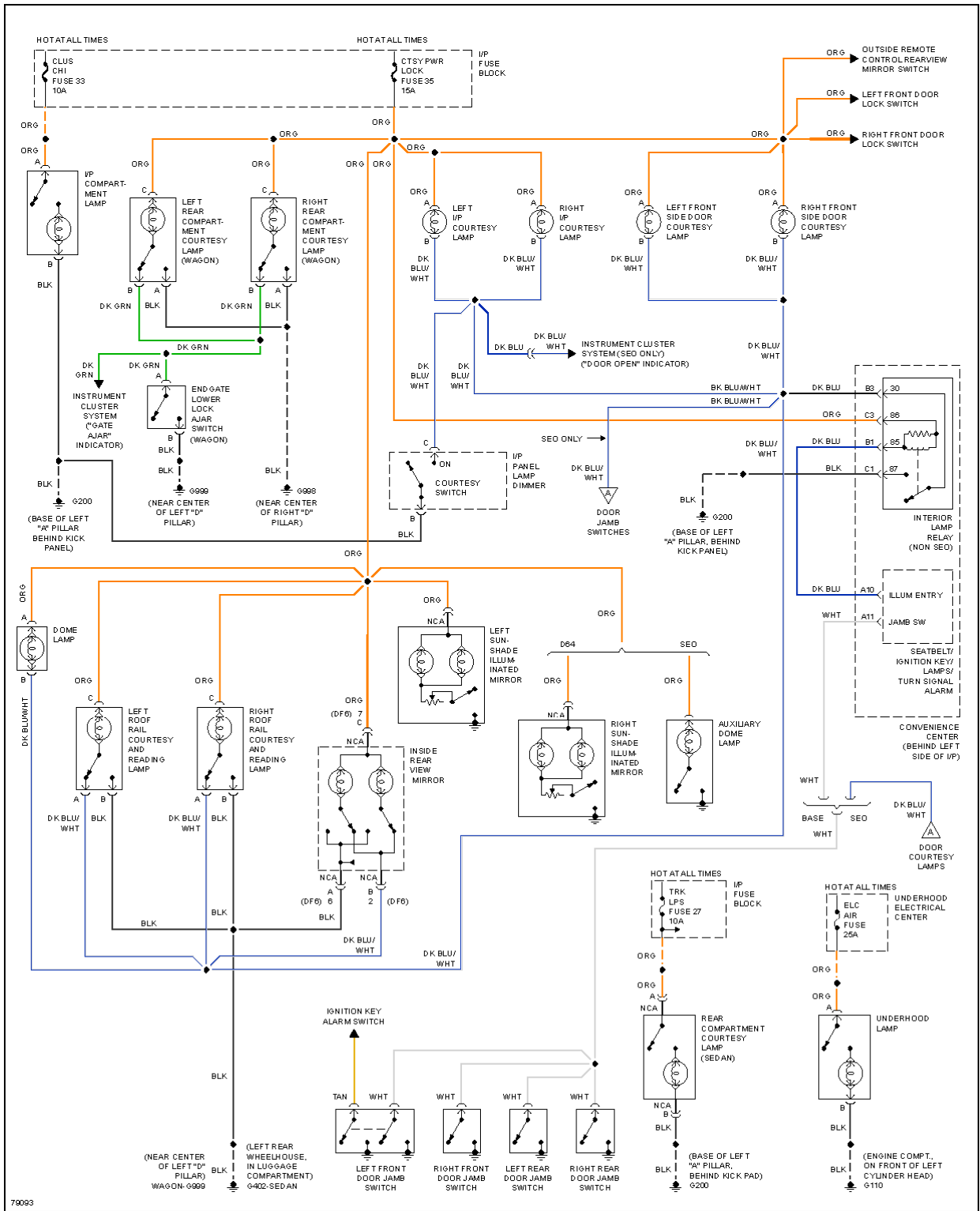
Fig. 24: Courtesy Lamps Circuit
