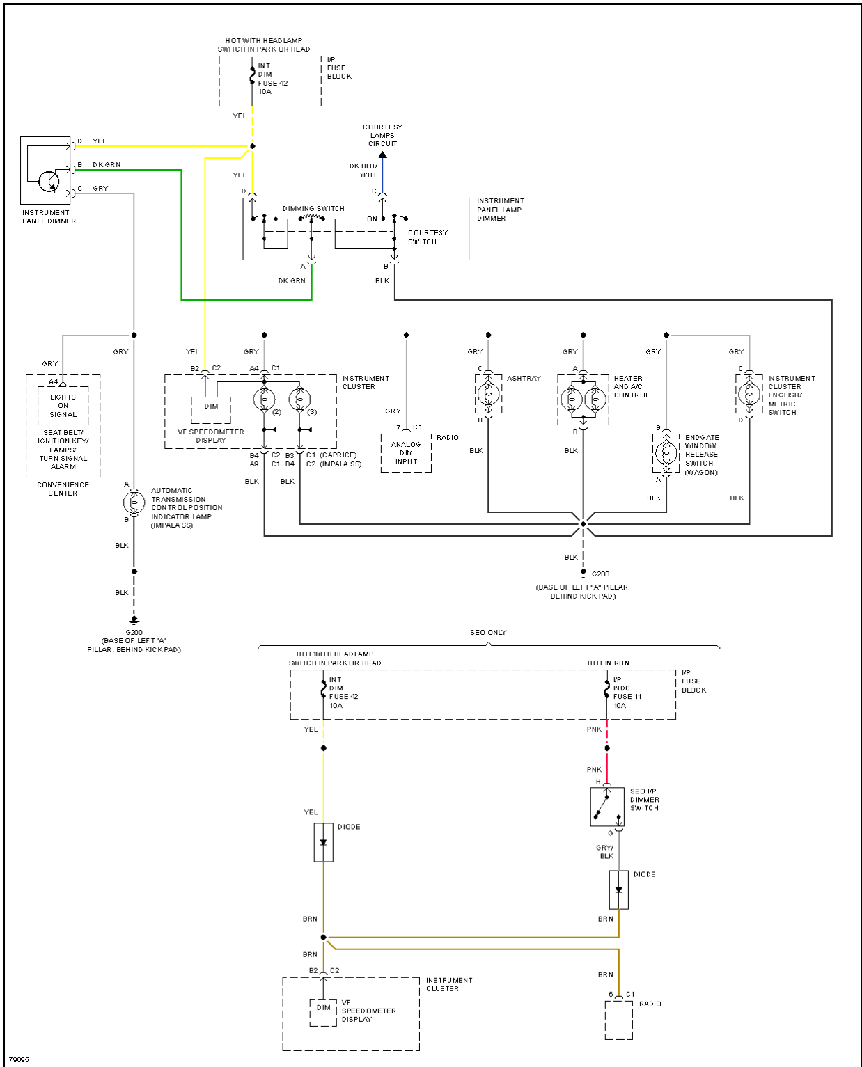
Fig. 25: Instrument Illumination Circuit
