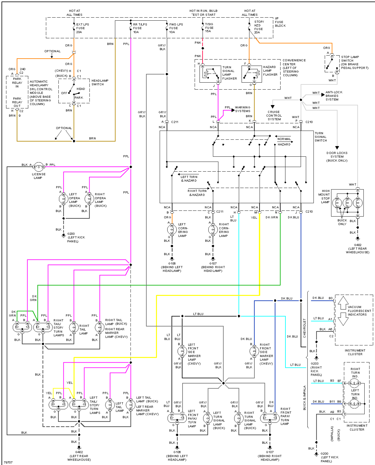
Fig. 14: Exterior Lamps Circuit, Sedan
