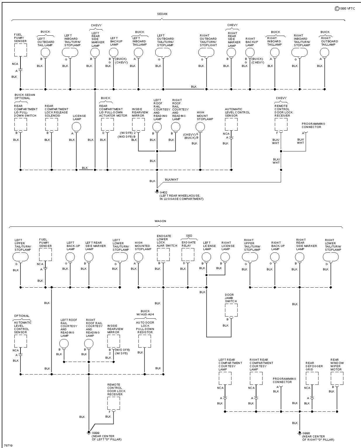
Fig. 17: Ground Distribution Circuit (3 of 3)
