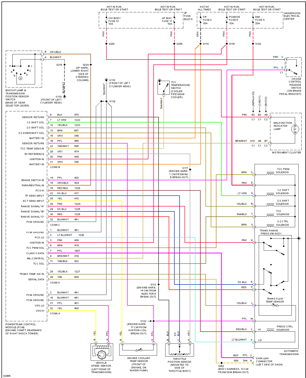
Fig. 40: 5.7L (VIN P), Transmission Circuit
