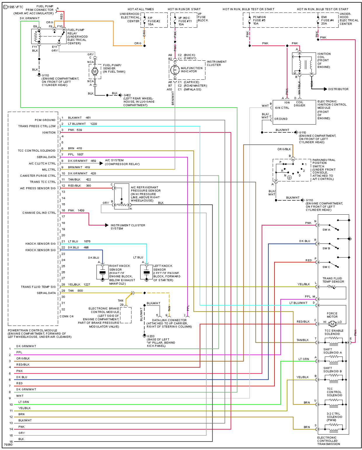
Fig. 11: 5.7L (VIN P), Engine Performance Circuits (3 of 3)
