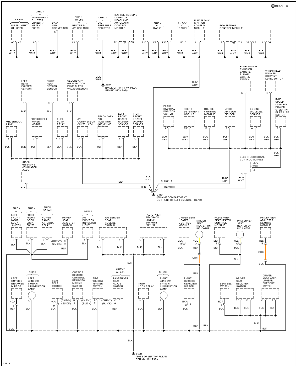
Fig. 16: Ground Distribution Circuit (2 of 3)
