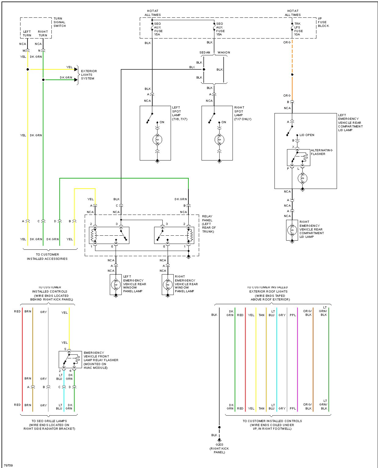
Fig. 12: Accessory Lamps Circuit
