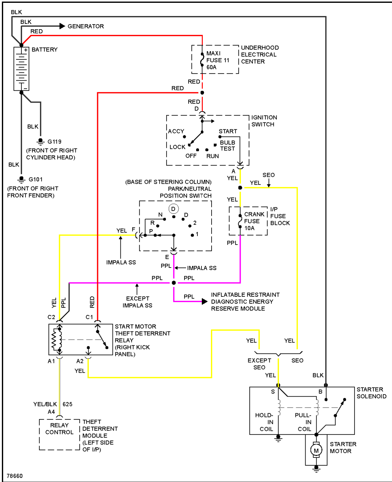
Fig. 38: Starting Circuit
