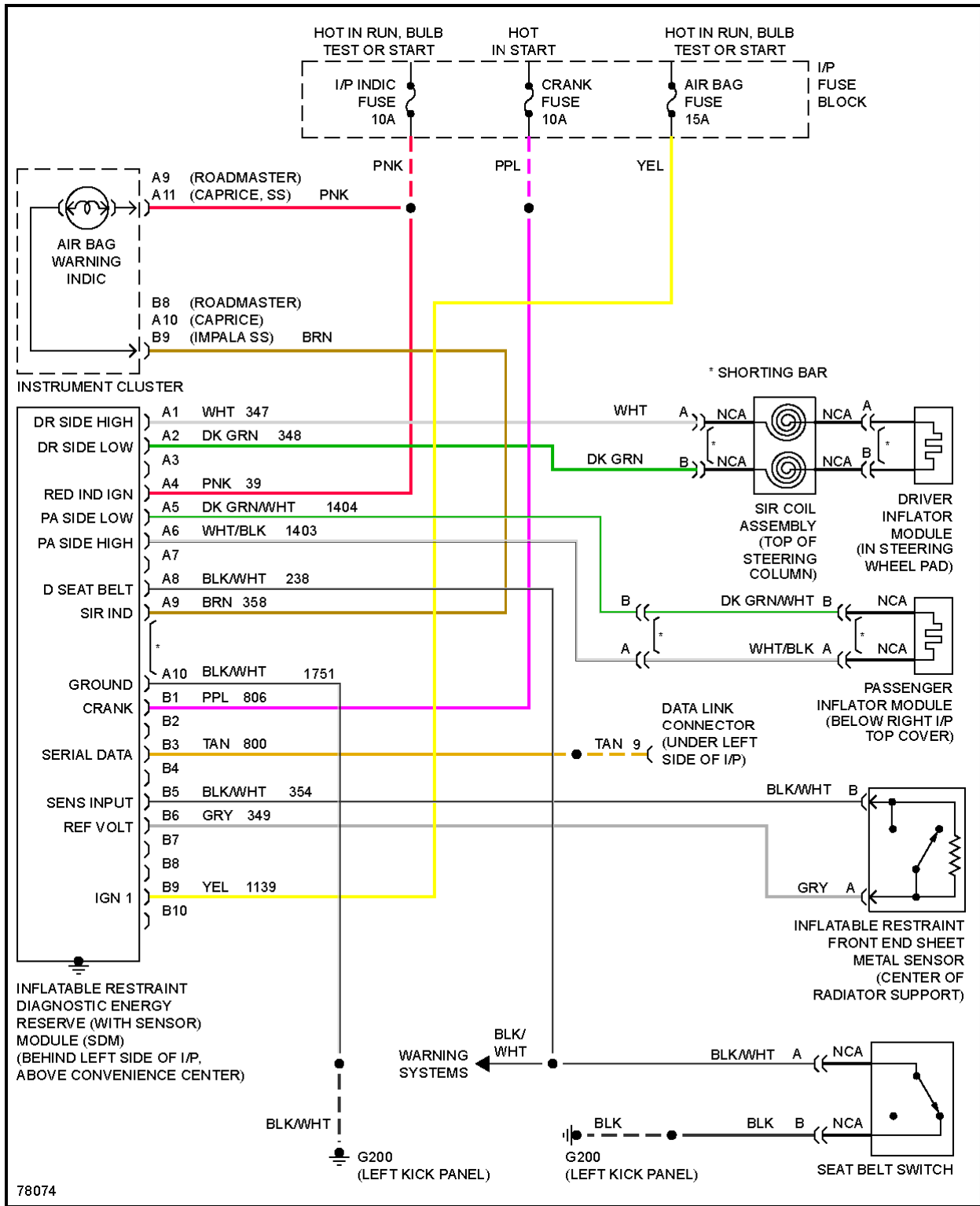
Fig. 39: Supplemental Restraint Circuit
