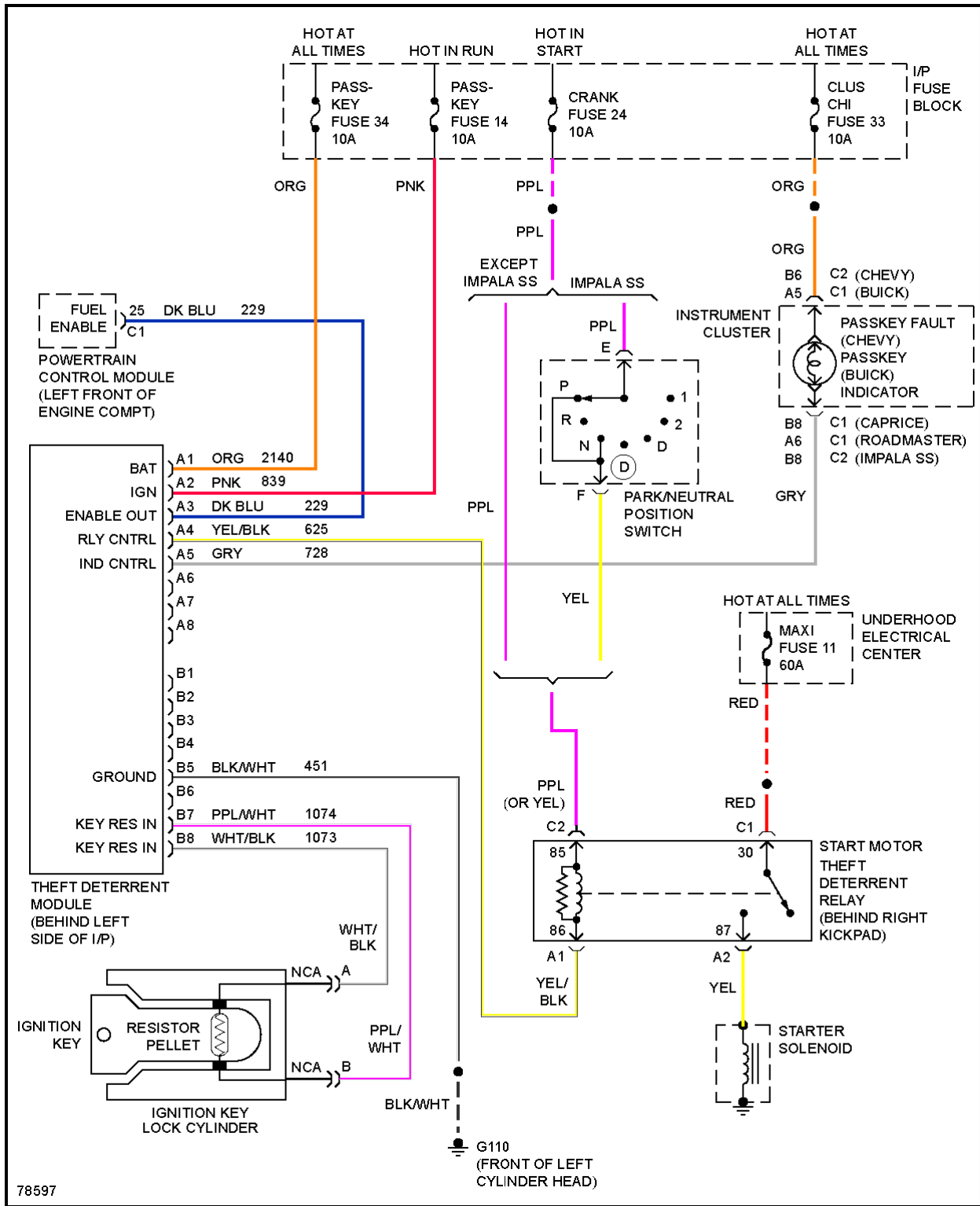
Fig. 4: Pass-Key Circuit, W/O SEO
