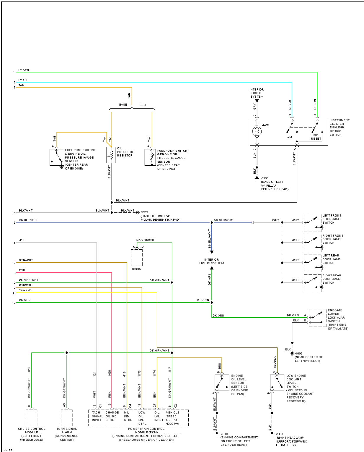
Fig. 23: Instrument Cluster Circuit (2 of 2)
