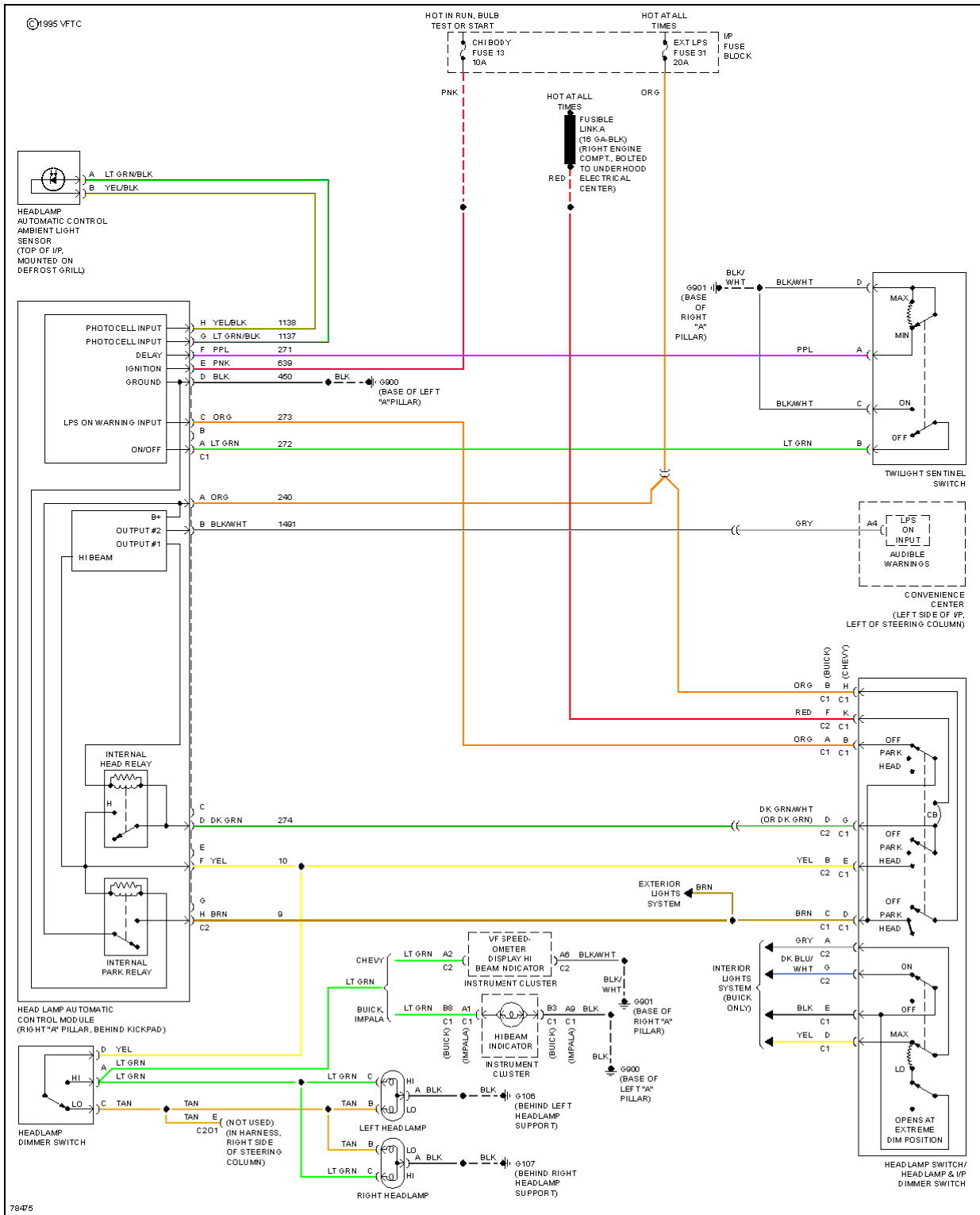
Fig. 19: Headlight Circuit, W/O DRL, W/ Twilight Sentinel
