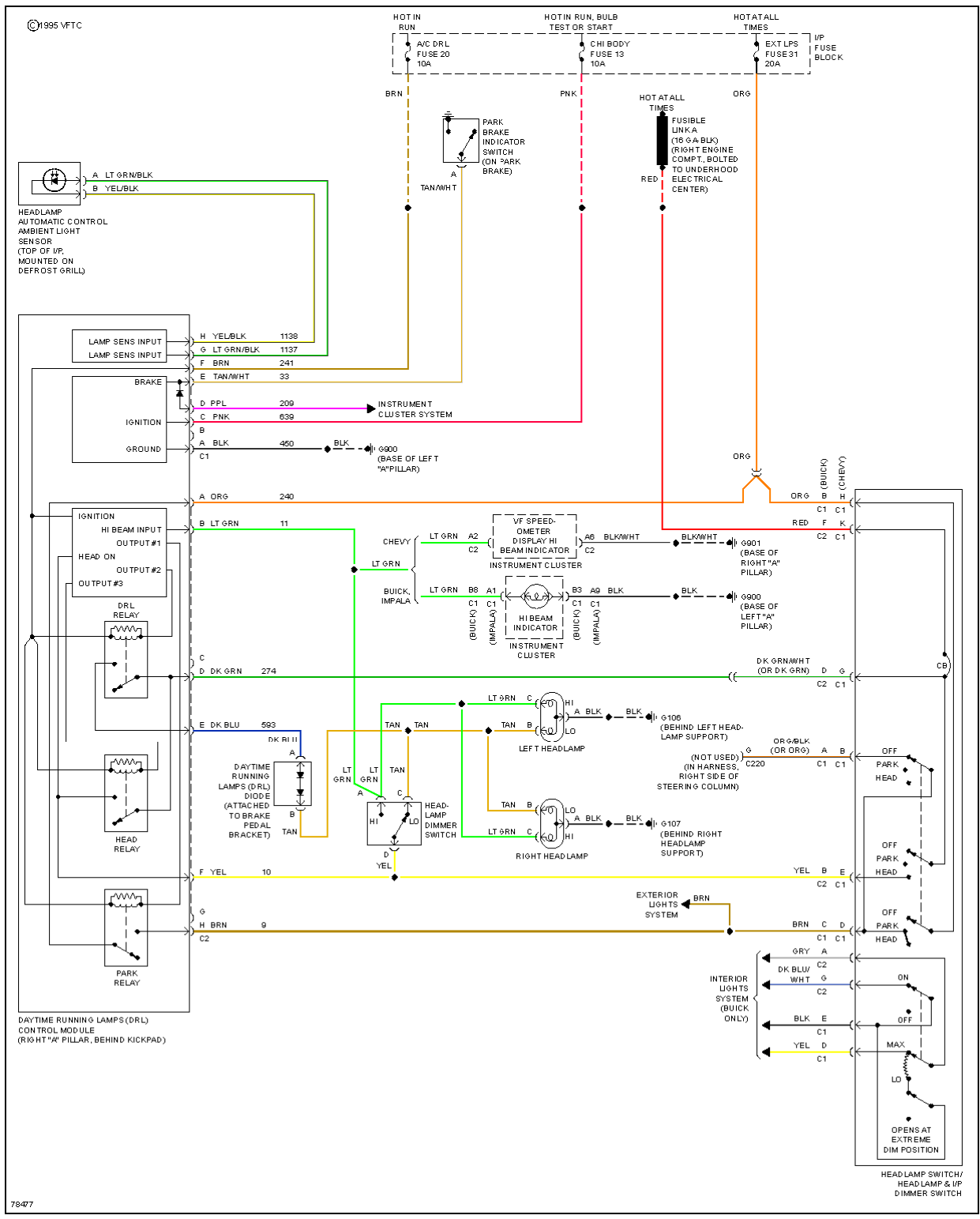
Fig. 18: Headlight Circuit, W/ DRL
