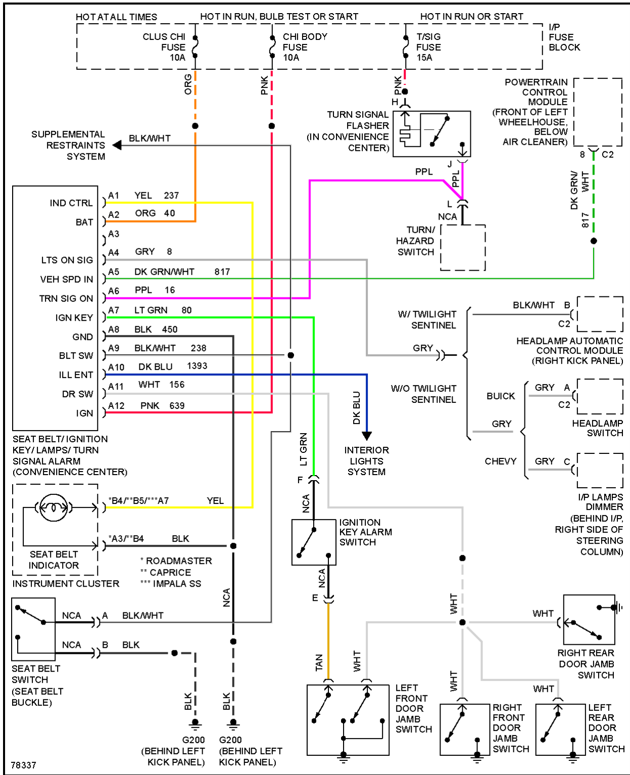
Fig. 43: Warning System Circuits
